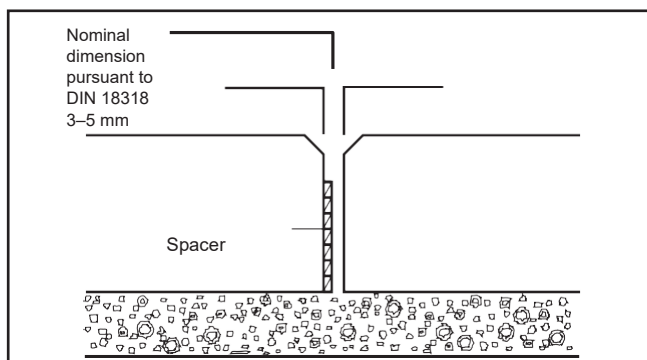
Correct joint formation: even when using spaces, the clinker bricks should not touch.
