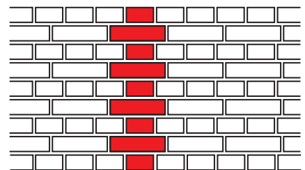
Blockverband
